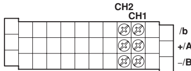
Input terminal block of the DX1002 and DX1002N
