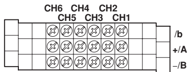
Input terminal block of the DX1006 and DX1006N
